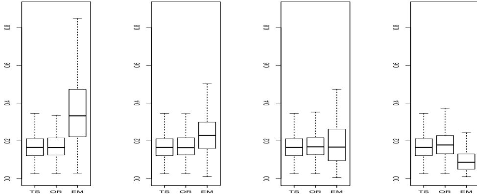
Figure 4: Boxplot of the L_1 -error for the estimate f_1^{em} (EM), the oracle estimate \bar{f}_1 (OR) and the two-step estimator \hat{f}_1 (TS) for the Laplace example. The separation distance \Delta between f_1 and f_2 vary from 0.1 (left) to 2 (right) and \ell_n = 5.5 .
