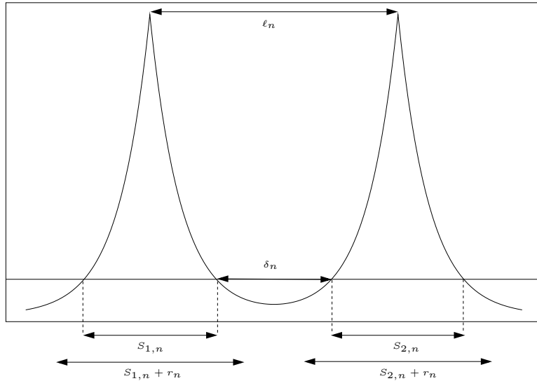
Figure 2: Connected components of level sets for a mixture of Laplace distributions.
