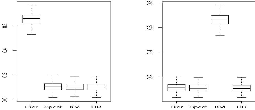
Figure 8: Boxplot of the L_1 -error for the oracle estimate \bar{f}_1 (OR) and two-step estimator \hat{f}_1 using the hierarchical algorithm (Hier), spectral clustering algorithm (Spect) and k -means algorithm (KM). Results are for “Circle-Square” dataset with a = 4 and n = 500 (left) and “Concentric circles” dataset with r_2 = 0.75 and n = 500 (right).
