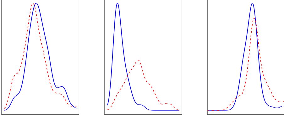
Figure 10: Kernel estimates \hat{f}_1^{(j)} (solid lines) and \hat{f}_2^{(j)} (dashed lines) for j = 1 (left), 2 (center) and 3 (right).
