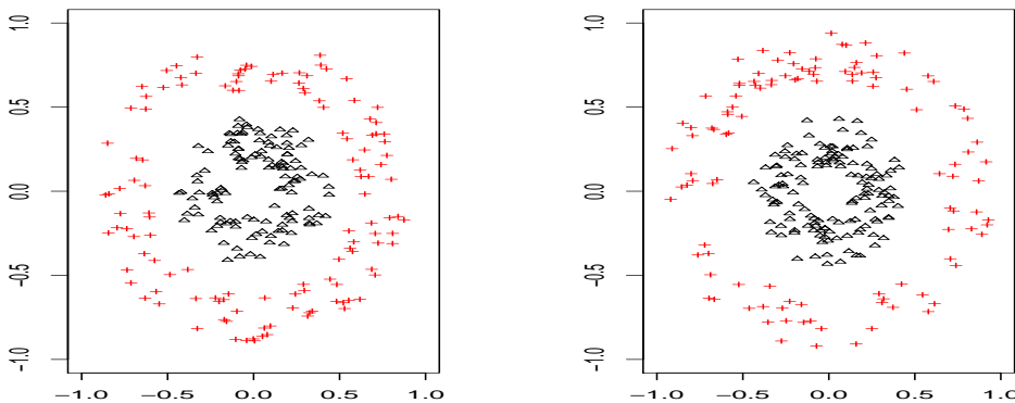
Figure 7: A sample of n = 250 observations for the “Concentric circles” model with r_2 = 0.75 (left) and r_2 = 0.80 (right).
