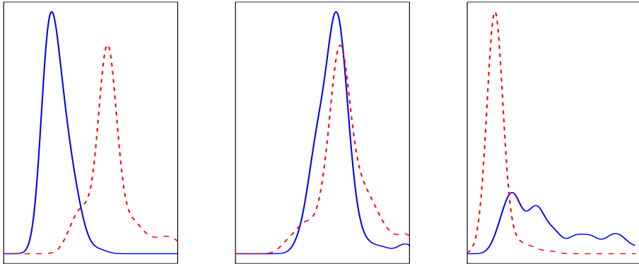
Figure 11: Kernel estimates \hat{f}_1^{(j)} (solid lines) and \hat{f}_2^{(j)} (dashed lines) for j = 4 (left), 5 (center) and 6 (right).
