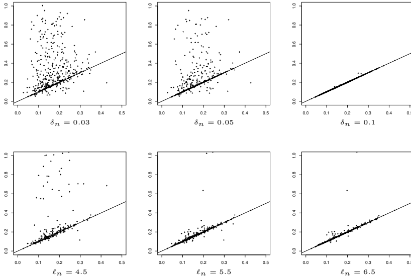
Figure 5: L_1 -error of \bar{f}_1 (x-axis) and \hat{f}_1 (y-axis) for the uniform (up) and Laplace (down) example.
