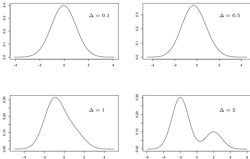
Figure 3: Density of Y for various values of \Delta .
