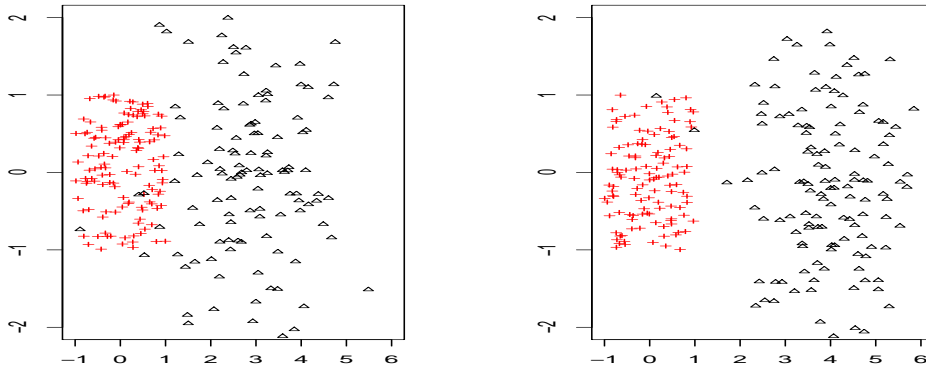
Figure 6: A sample of n = 250 observations for the “Circle-Square” model with a = 3 (left) and a = 4 (right).
