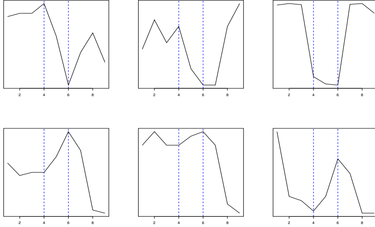
Figure 9: Consumptions of users suspected to be affected (up) or not (down) by the perturbation.
